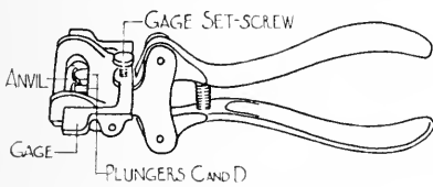
FIG. 109. SAW SET.
